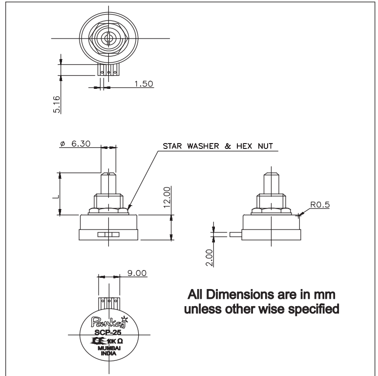
Dimensional Diagram
