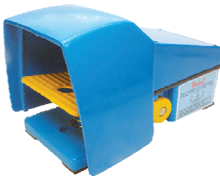
Foot Operated Potentiometer Model: FOP-D Dome Shape Cover
