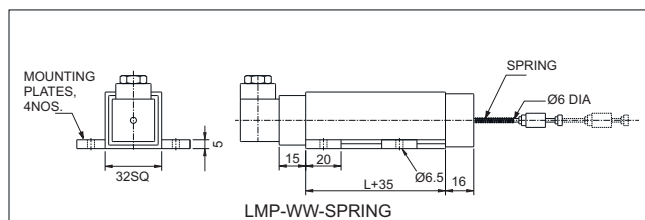
External Spring Return
