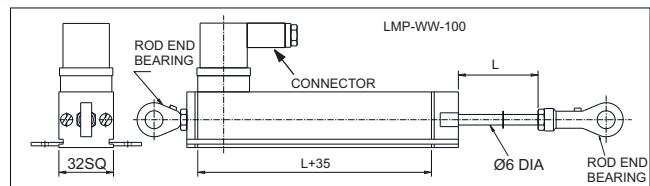
Rod End Bearing on Both Side
